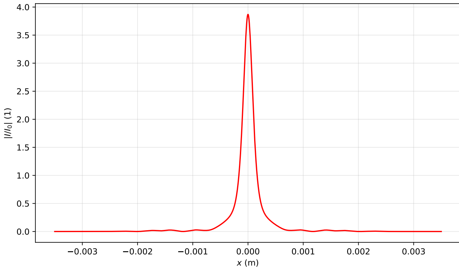
Intensity profile I(x, y = 0, z = 2.149)/I_0 , P_{in}=3.5P_{cr} , artificial time
